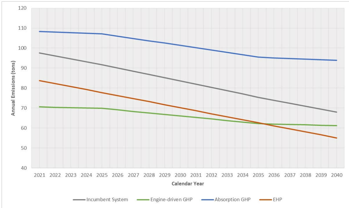
Figure 18: Estimated Annual Carbon Emissions of Cooling and Heating from 2021-2040 at Stand-Alone Retail Stores in Las Vegas
