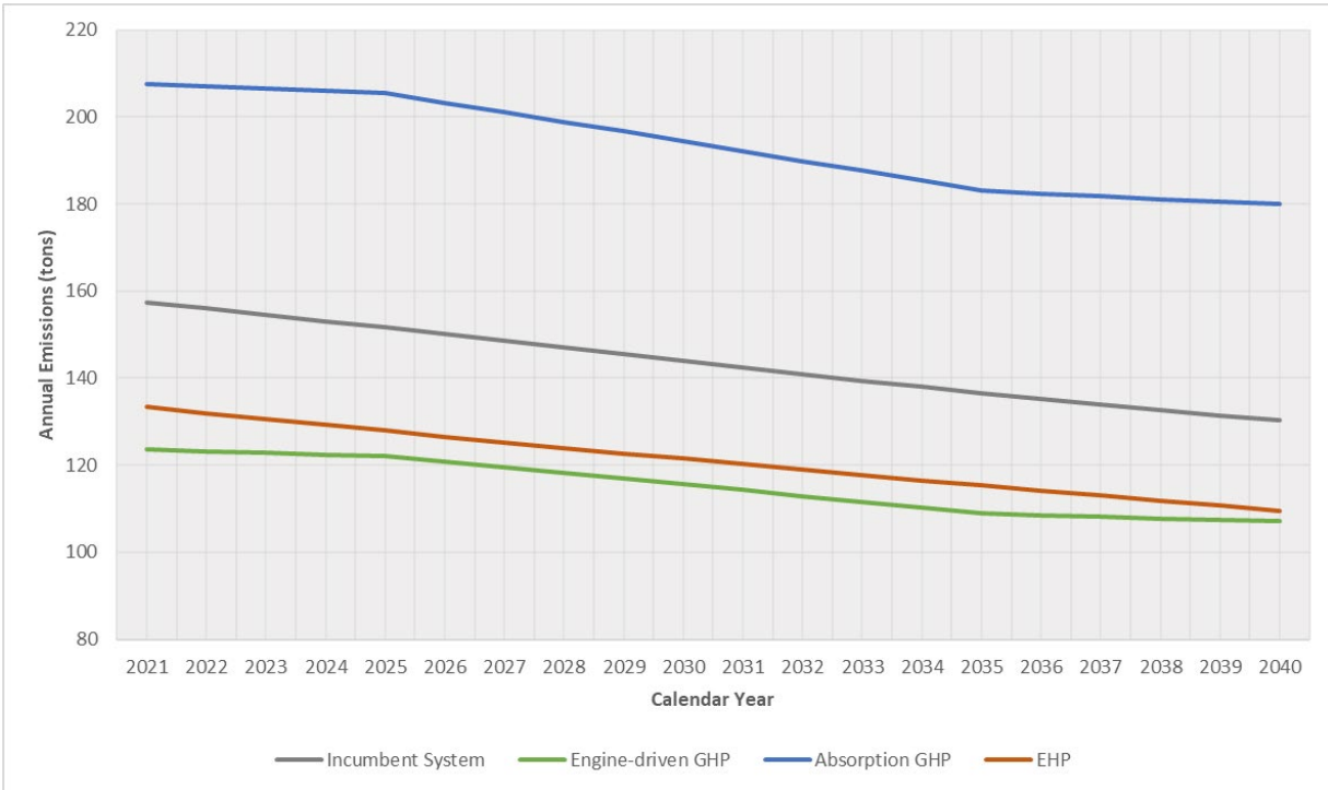
Figure 16: Estimated Annual Carbon Emissions of Heating and Cooling from 2021-2040 in Medium-sized Offices in Houston
