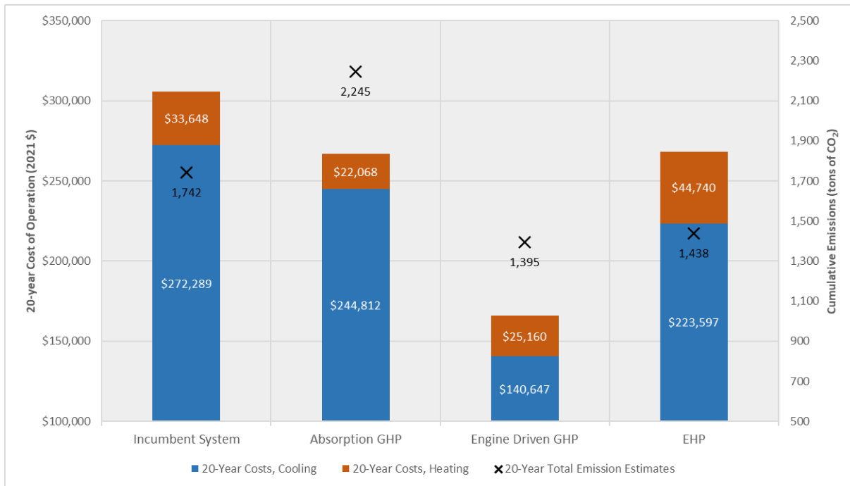
Figure 13: 20-year Operating Costs and Emission Estimates of Heating and Cooling at Stand-Alone Retail Stores in Houston
