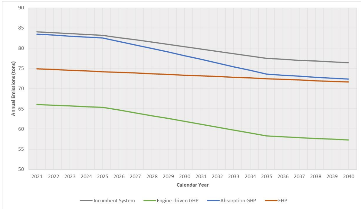
Figure 10. Estimated Annual Carbon Emissions of Heating and Cooling from 2021-2040 in Stand-Alone Retail Stores in Baltimore
