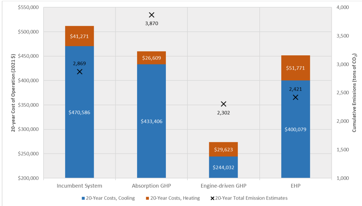
Figure 15: Estimated Annual Carbon Emissions of Heating and Cooling at Medium-sized Offices in Houston
