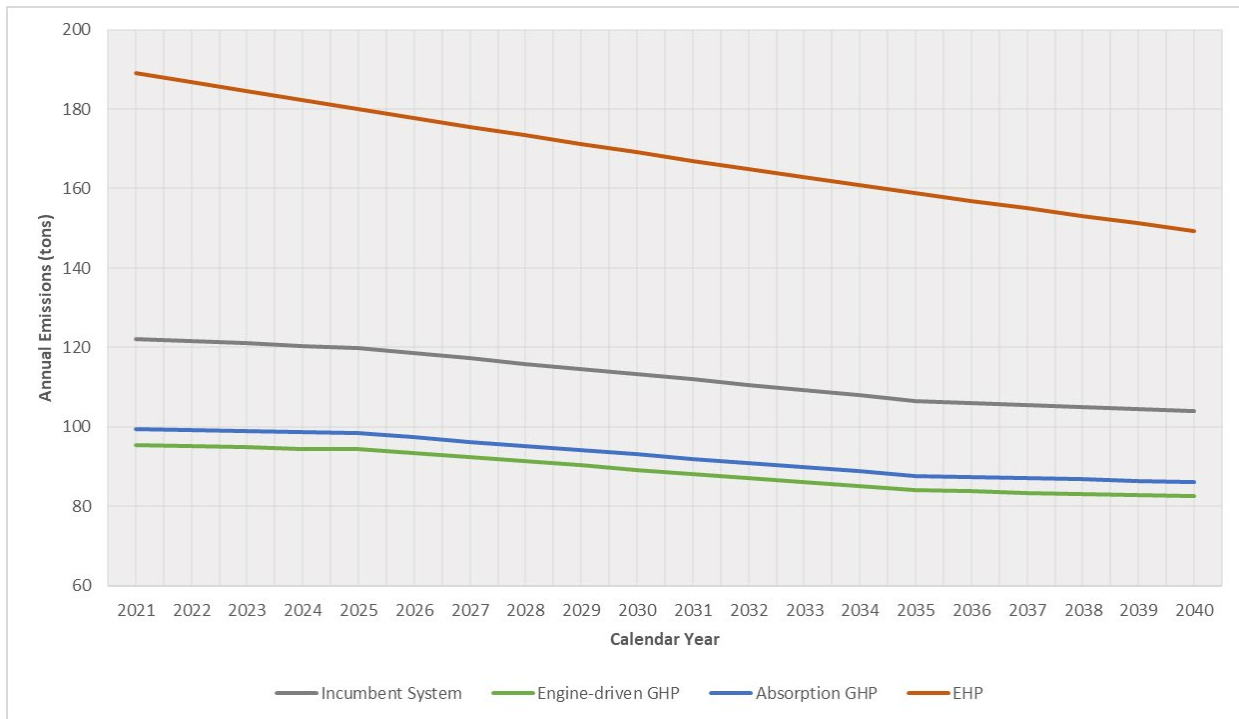
Figure 22: Estimated Annual Carbon Emissions of Heating and Cooling from 2021-2040 at Stand-Alone Retail Stores in Minneapolis
