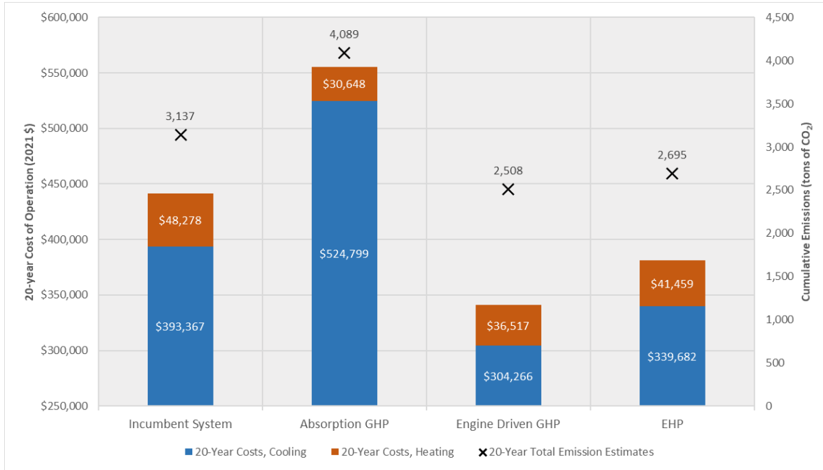
Figure 19: 20-year Operating Costs and Emission Estimates of Heating and Cooling at Medium-sized Offices in Las Vegas
