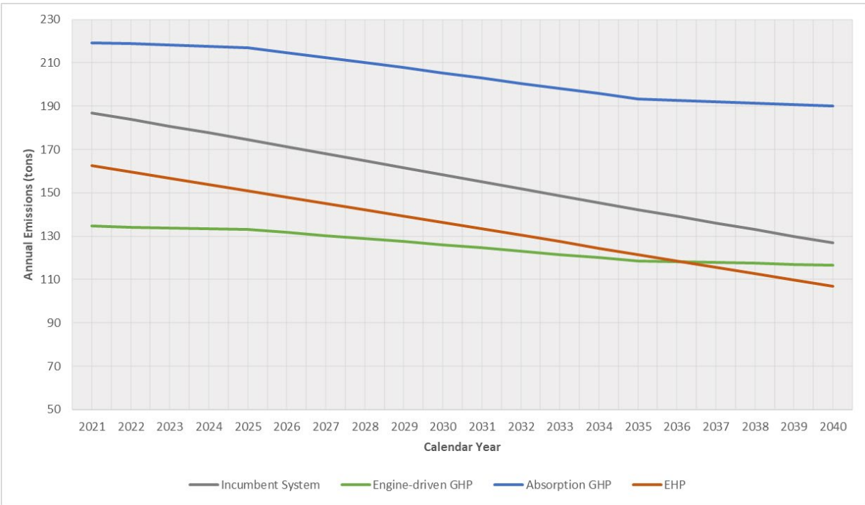
Figure 20: Estimated Annual Carbon Emissions of Heating and Cooling from 2021-2040 at Medium-sized Offices in Las Vegas
