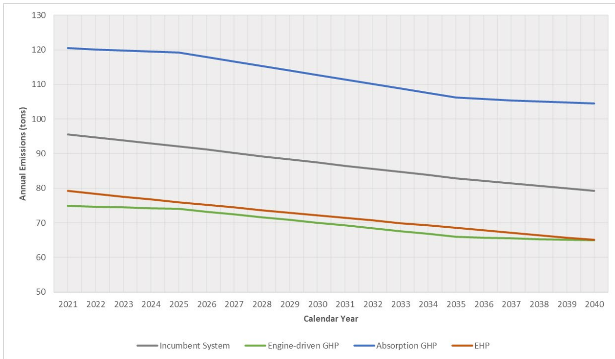
Figure 14: Estimated Annual Carbon Emissions of Heating and Cooling from 2021-2040 at Stand-Alone Retail Stores in Houston
