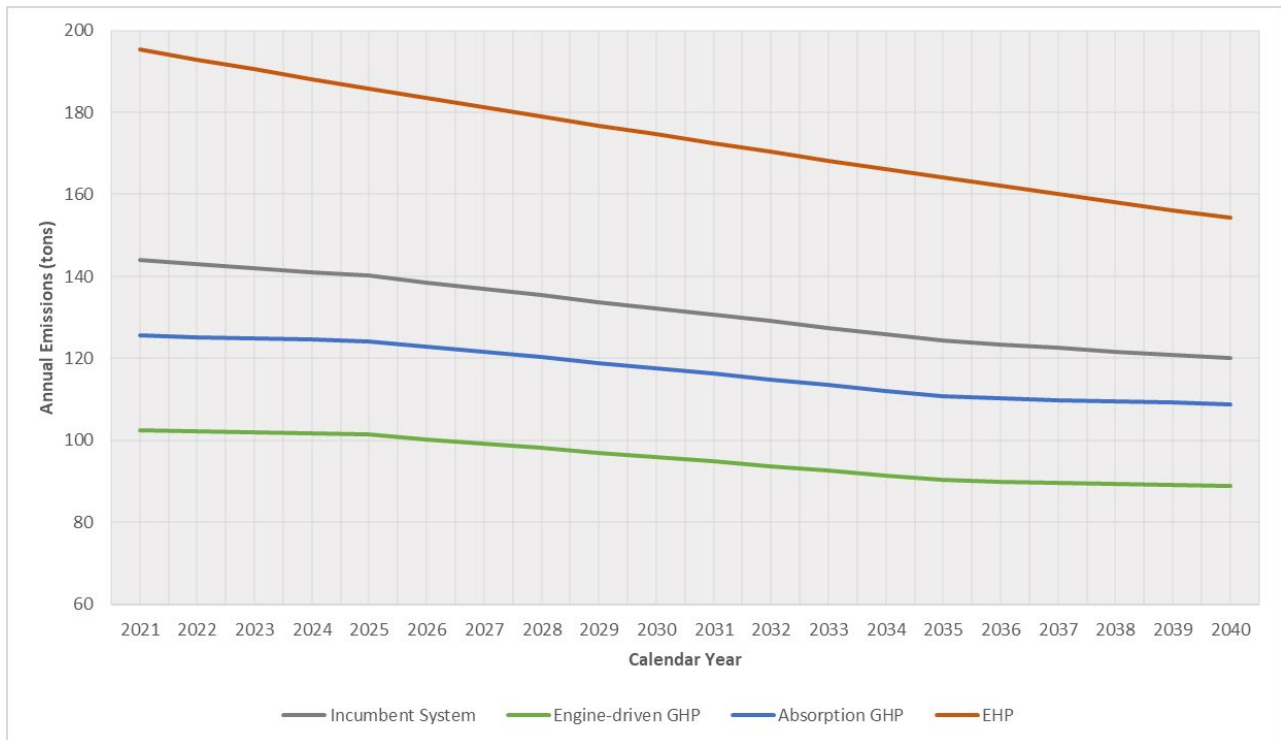
Figure 24: Estimated Annual Carbon Emissions of Heating and Cooling from 2021-2040 at Medium-sized Offices in Minneapolis
