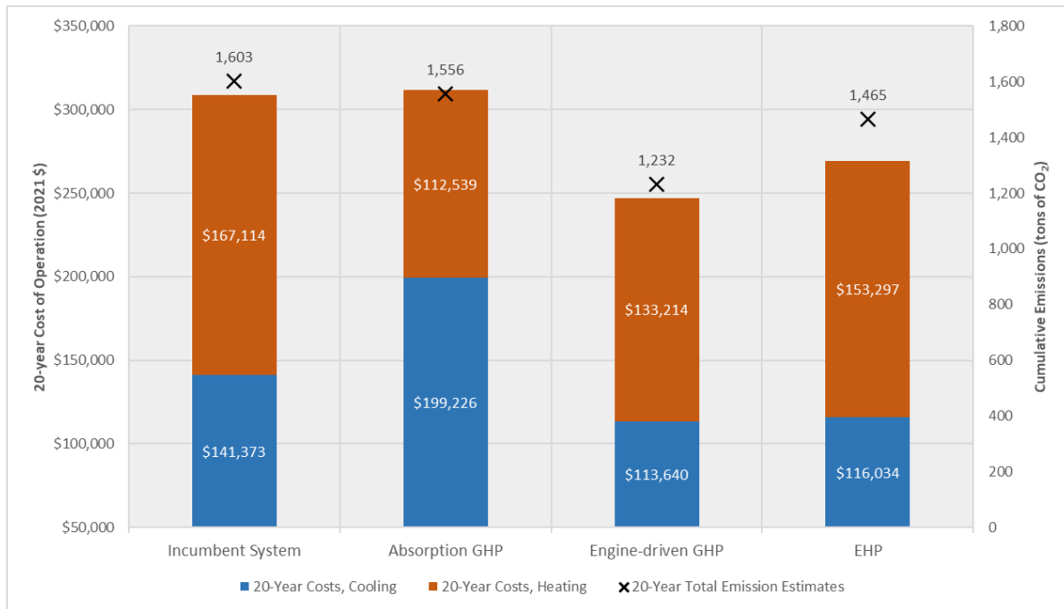
Figure 9. 20-year Operating Costs and Emission Estimates of Heating and Cooling in Stand-Alone Retail Stores in Baltimore
