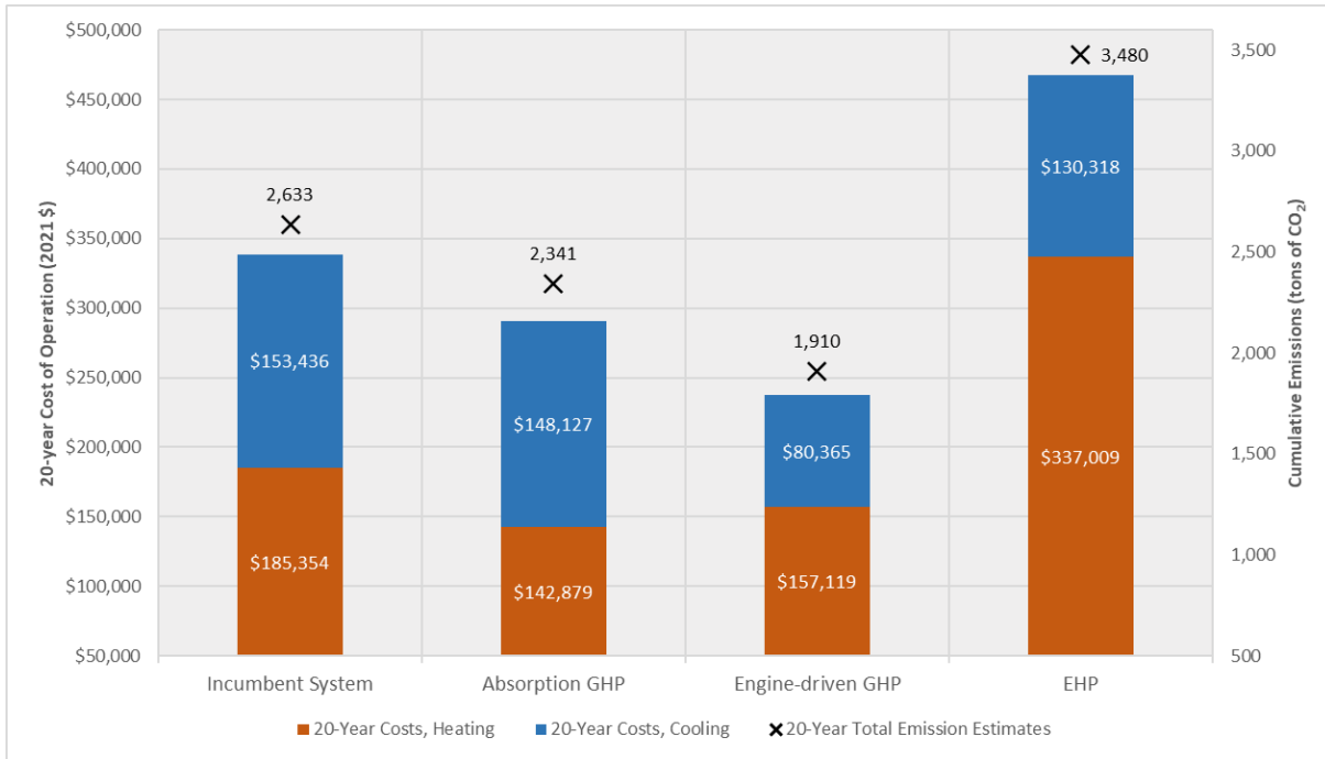
Figure 23: 20-year Operating Costs and Emission Estimates of Heating and Cooling in Medium-sized Offices at Minneapolis
