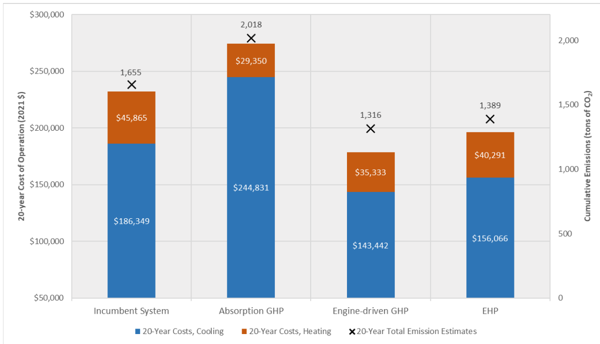
Figure 17: 20-year Operating Costs and Emission Estimates of GHPs at Stand-Alone Retail Stores in Las Vegas
