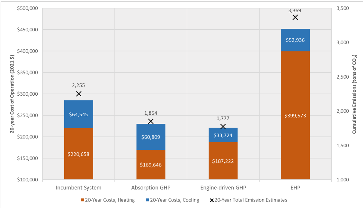
Figure 21: 20-year Operating Costs and Emission Estimates of Heating and Cooling at Stand-Alone Retail Stores in Minneapolis
