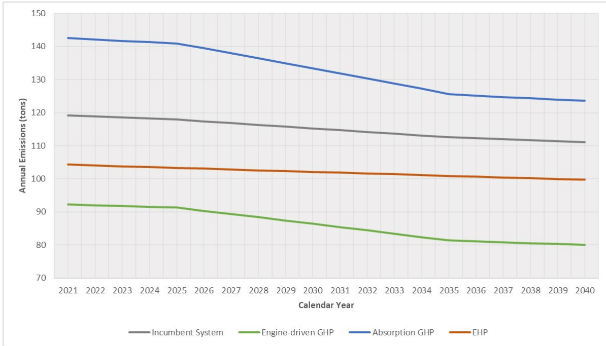
Figure 12: Estimated Annual Carbon Emissions of Heating and Cooling from 2021-2040 in Medium-sized Offices in Baltimore
